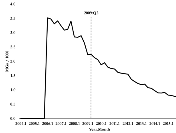
f: Meperidine
