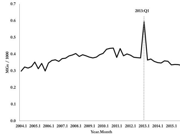
d: Fentanyl
