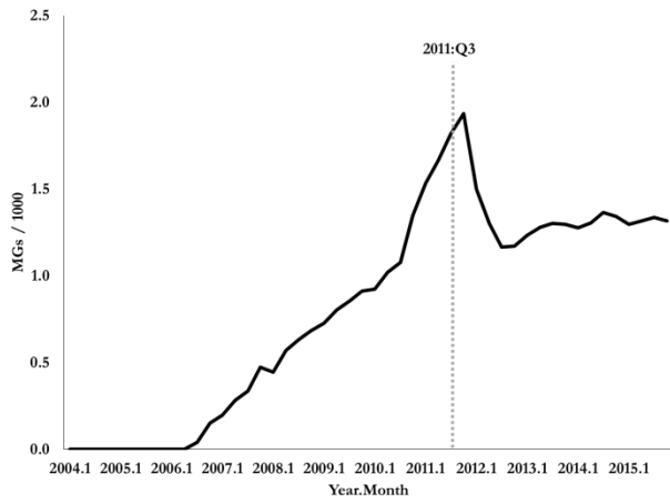
e: Oxymorphone
