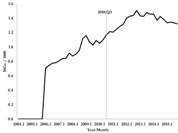
g: Hydromorphone
