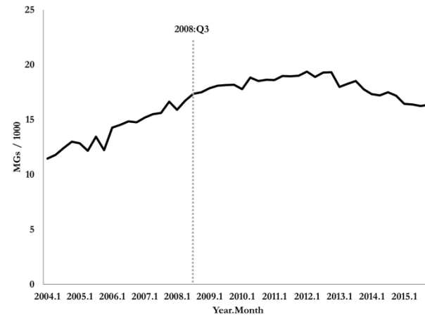
b: Morphine
