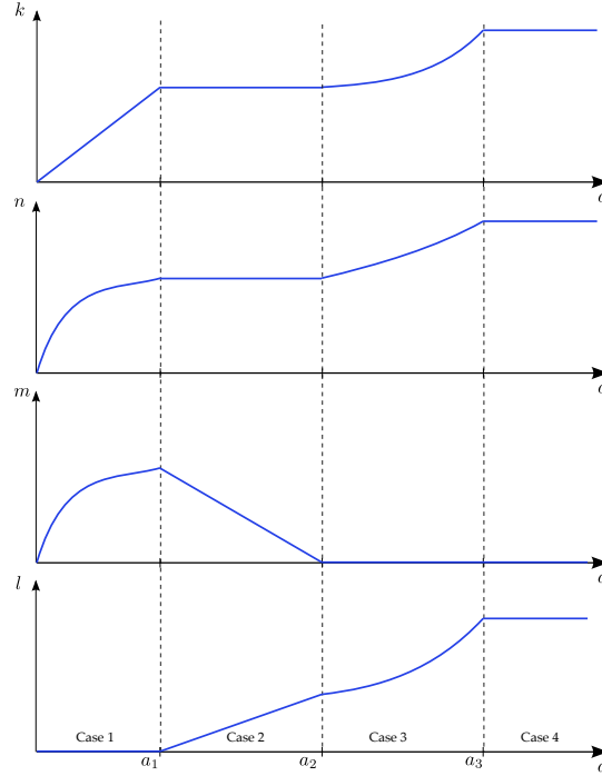
Figure 10: Solution to the firm problem
