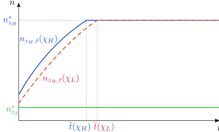
Figure 3: Firm employment dynamics: comparative statics with respect to \chi
