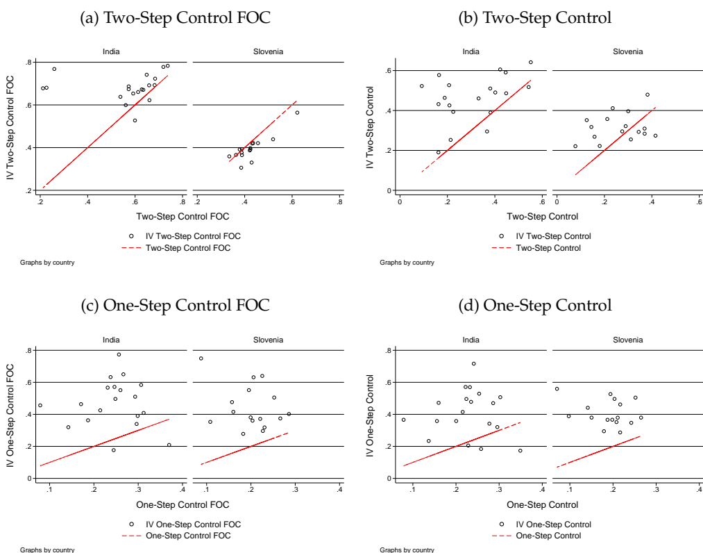
Figure 3: Industry-specific Coefficients
