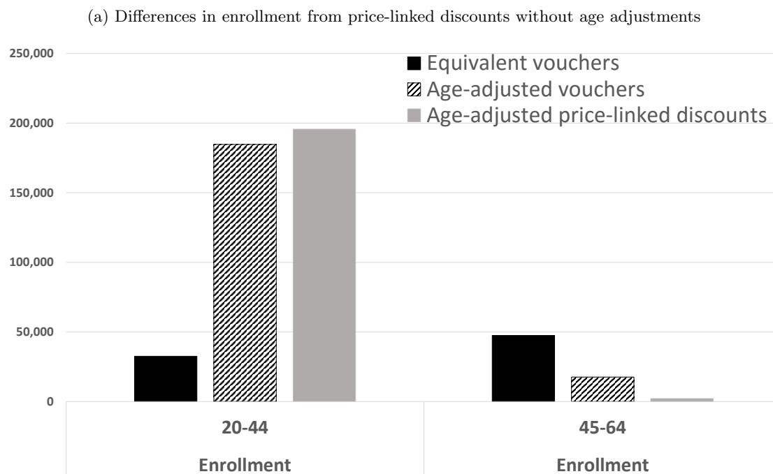
Figure 10: Summary of differences between ACA scheme and counterfactual alternatives
