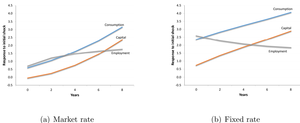
Figure 20: Responses of Endogenous Variables to a Labor-Force Shock
