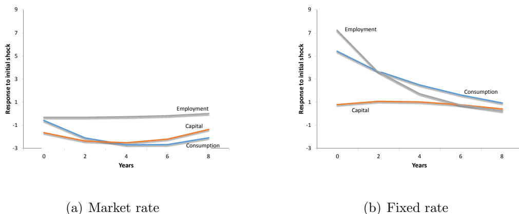
Figure 19: Responses of Endogenous Variables to a Discount Shock
