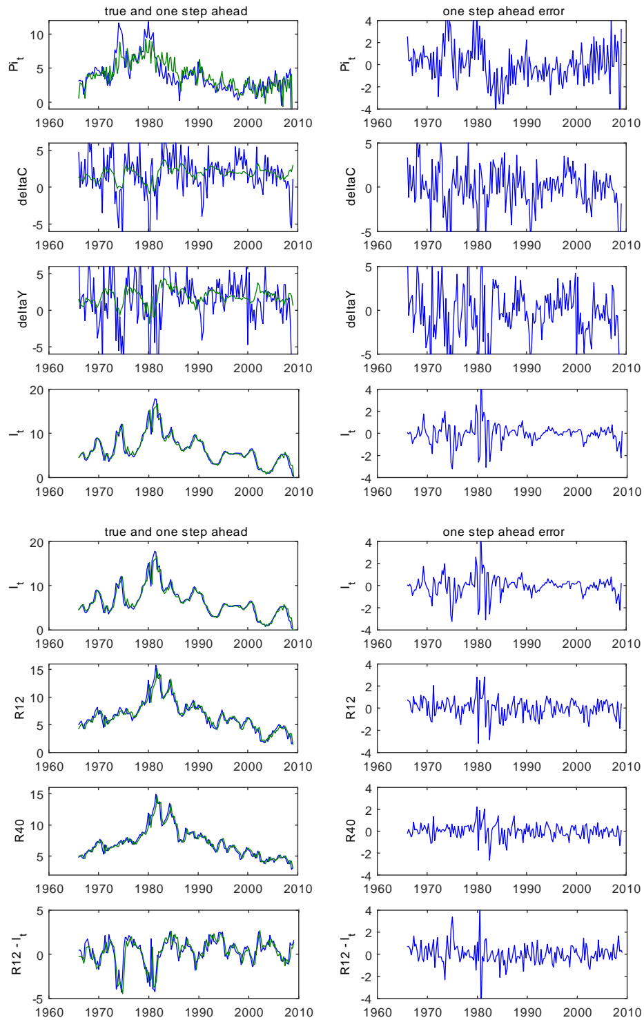
Figure 4: Actual and 1-step ahead forecasts
