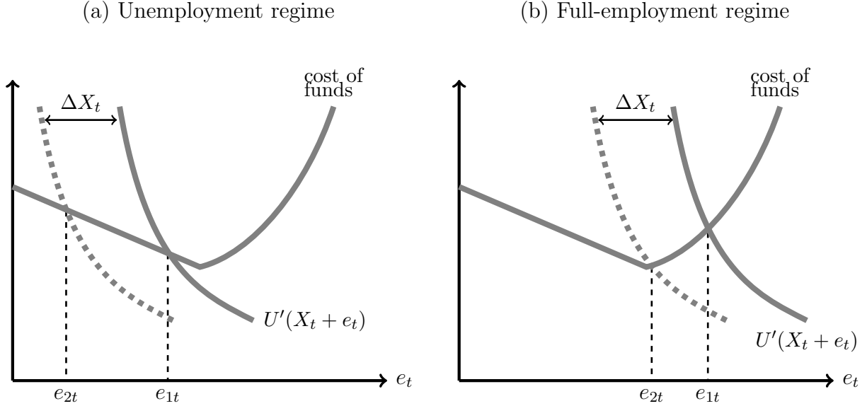
Figure 4: Period t Equilibrium Determination in the Myopic Model
