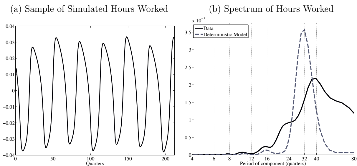
Figure 7: Deterministic Model
