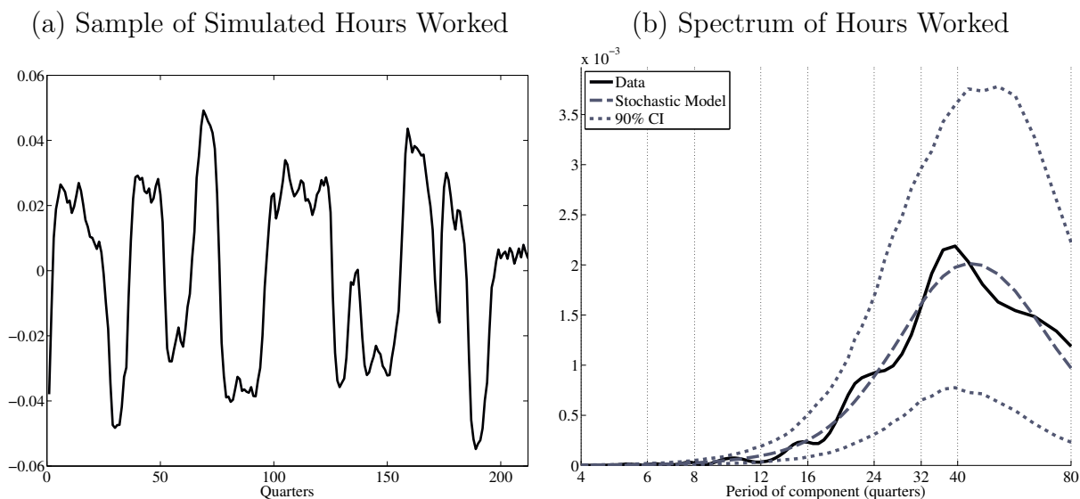
Figure 8: Stochastic Model
