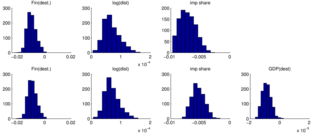
Figure 5: Histograms of regression coefficients from two regressions performed on randomly generated data. The artificial data samples are counterfactual shadow tax rates computed as follows: keeping the diagonal elements of the international portfolio of each country fixed, we re-shuffle the elements of the international portfolio holdings of each country in a random manner. We create 1000 artificial portfolio matrices and compute 1000 artificial tax rates. For each draw, we regress the difference between the tax rates we obtain from actual data ( \tau_{ij} ) and the artificial tax rates corresponding to the random draw ( \tau_{ij}^* ) on \tau_{ij}^* , the size of the financial industry of both destination and origin country, log distance between the two countries, and the import shares as described in the text. The histograms for the coefficients on the destination country’s industry, log distance, and import shares are given by the top three histograms. The lower histograms report results of the same regression, but including the GDP of destination and origin country as additional regressors.
