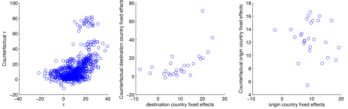
Figure 4: Scatter-plot of implied tax rates versus counter-factual implied tax rates. The counter-factual implied tax rates are computed by assuming that domestic investors’ portfolio allocation to domestic risky asset is unchanged. However, the fraction of the portfolio that is invested internationally is invested as if there were no frictions. The left plot depicts all N^2 implied tax rates. The middle plot depicts the estimated destination-country fixed-effects for actual and counterfactual implied tax rates. The right plot depicts the estimated origin-country fixed-effects for actual and counterfactual implied tax rates.
