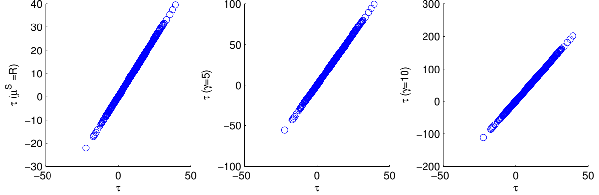
Figure 6: Left plot: Scatterplot of our implied tax rates (x-axis) versus implied tax rates imposing \mu^S = R (y-axis). Middle and right plots: Scatterplots of our implied tax rates (x-axis) versus implied tax rates resulting when \gamma = 5 , respectively \gamma = 10 (y-axis).
