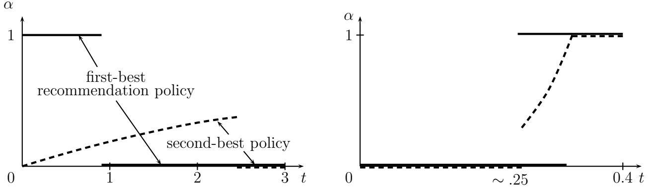
Figure 1: Path of \alpha for \Delta > 0 (left panel, (c, \mu, p_0, r, \lambda_g, \lambda_b) = (2/3, 1/4, 1/2, 1/10, 4/5, 0) ) and \Delta < 0 (right panel, (c, \mu, p_0, r, \lambda_g, \lambda_b) = (1/2, 1, 2/7, 1/10, 1, 2) )
