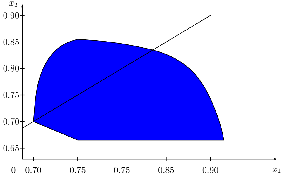
Figure 4: Region B_2 of feasible (x_1, x_2) in the case J = 2 (here, for \ell_0 = 5, \ell_1 = 3, \ell_2 = 2, \mu_1 = 2/3 ).
