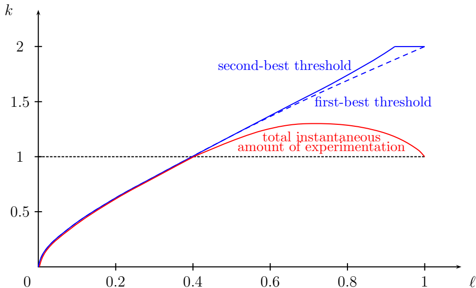
Figure 2: Optimal policy with a continuum of cost levels (here, \bar{k} = 2, \ell_0 = 1 ).
