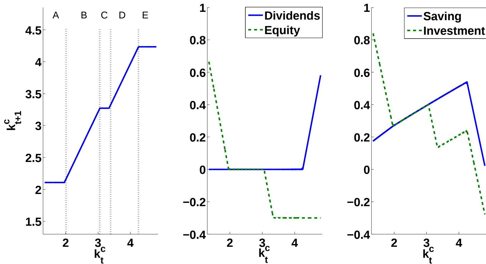
Figure 12: Policy Functions
