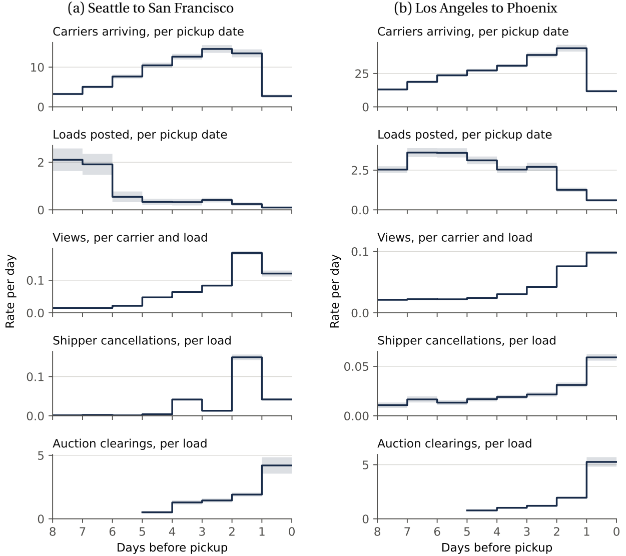
Figure D.1: Estimated arrival rates of the platform's events
