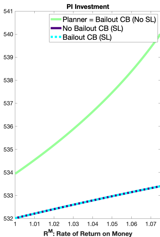
Figure 15: Welfare Decomposition
