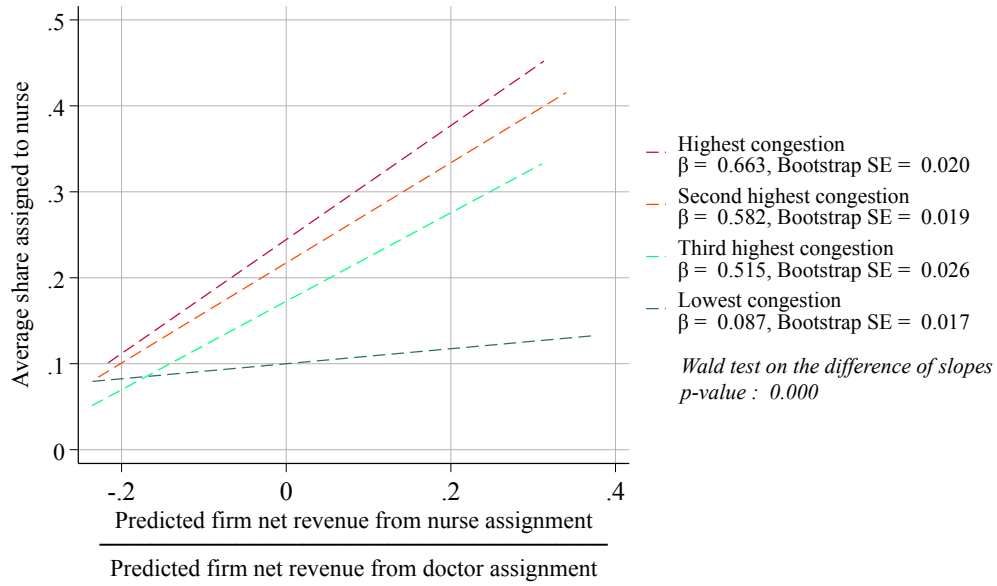
(a) Relative firm net revenue advantage
