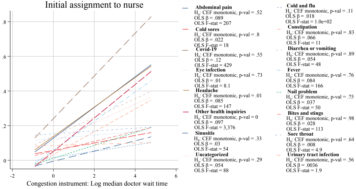
Figure A10. Instrument monotonicity test
