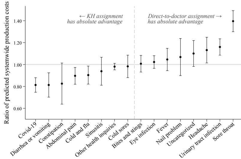
(a) Comparative advantage
