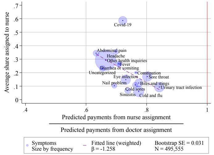
(b) Taxpayer payments to the firm
