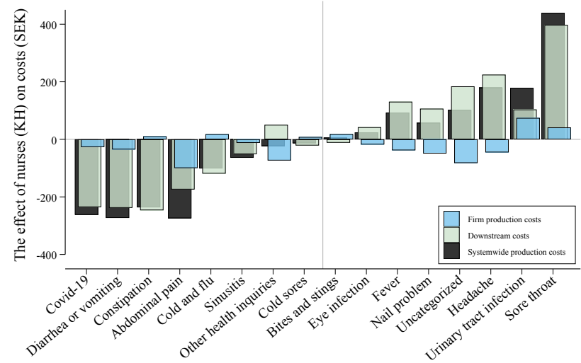
(b) Breakdown of systemwide production costs
