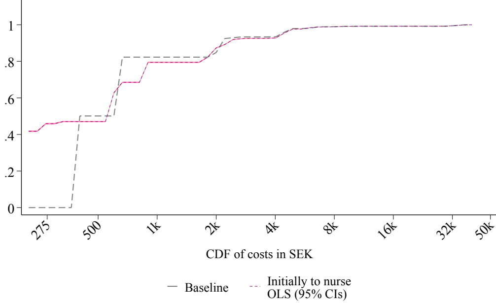
(b) Distribution of systemwide production costs
