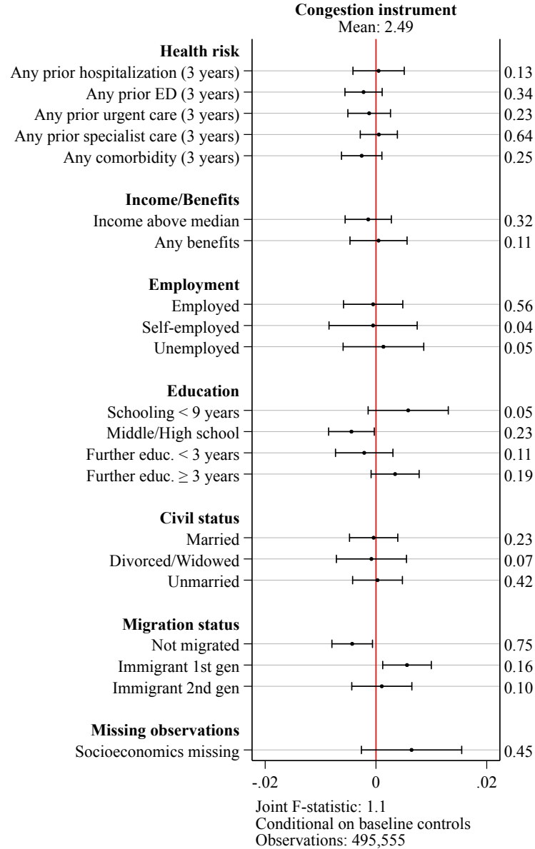
Figure A9. Balance of the congestion instrument in case characteristics
