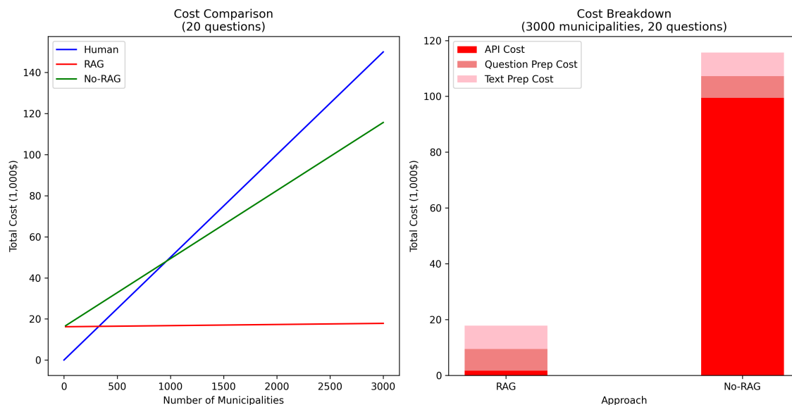
Figure A3: Comparison of Human vs. LLM Cost
