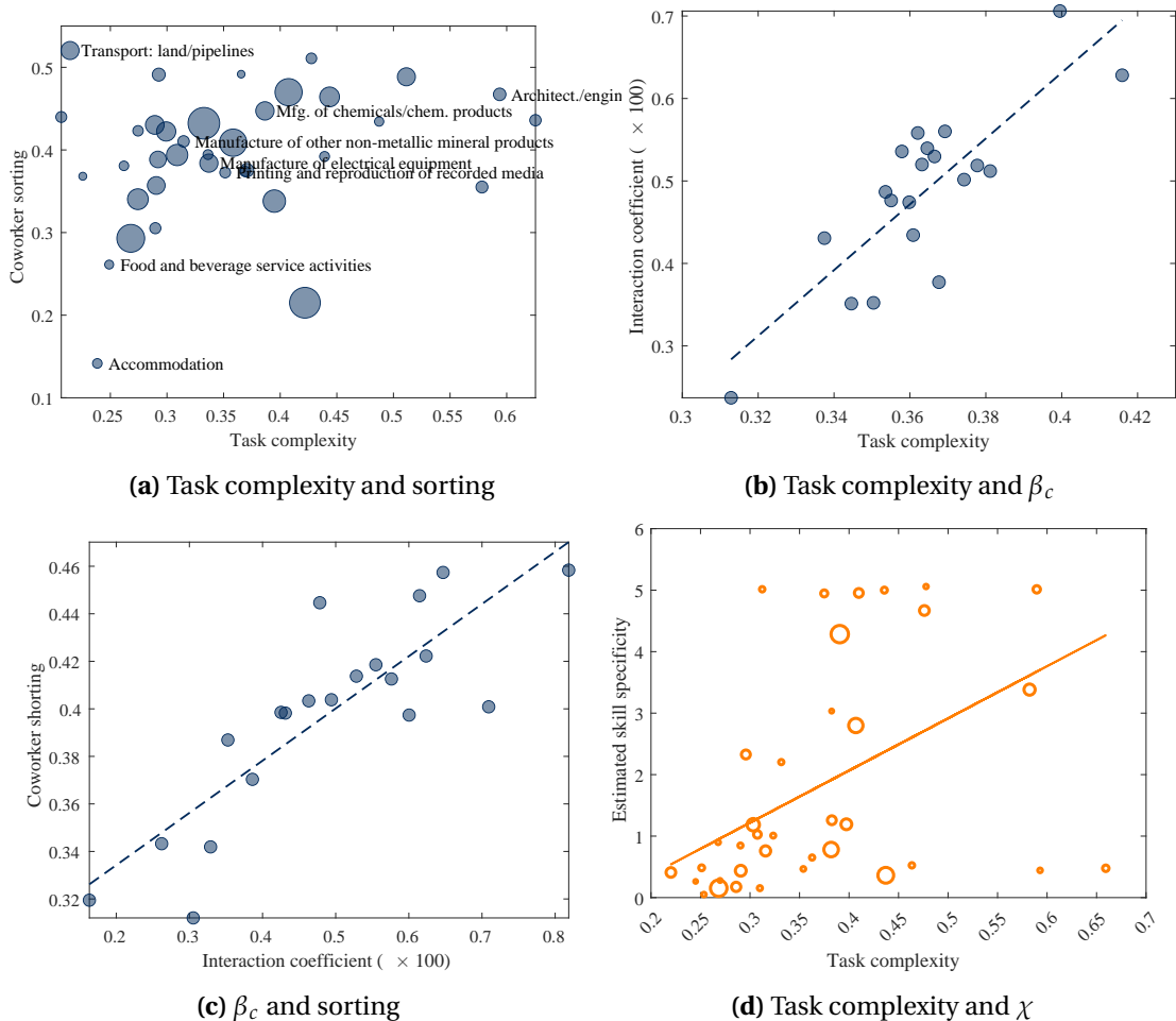
Figure 6: Industry-level evidence
