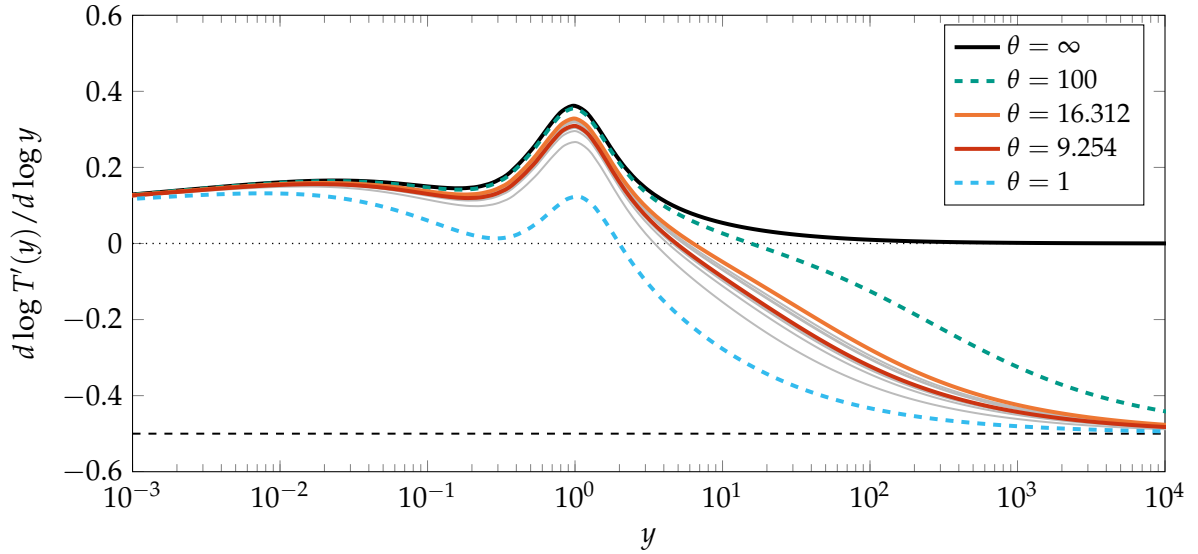
Figure 6: Growth rates of optimal marginal tax schedules, d \log T'(y) / d \log y , for alternative levels of misspecification concerns. The dashed black line corresponds to the theoretical limit, equal to -1/2 .
