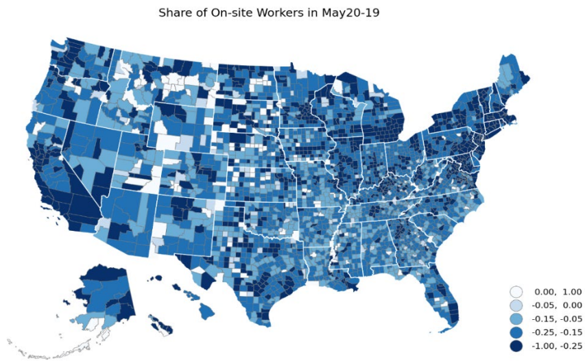
Figure 3: Difference in Share of Workers Persisting in Onsite Work from February, May 2020 minus May 2019
