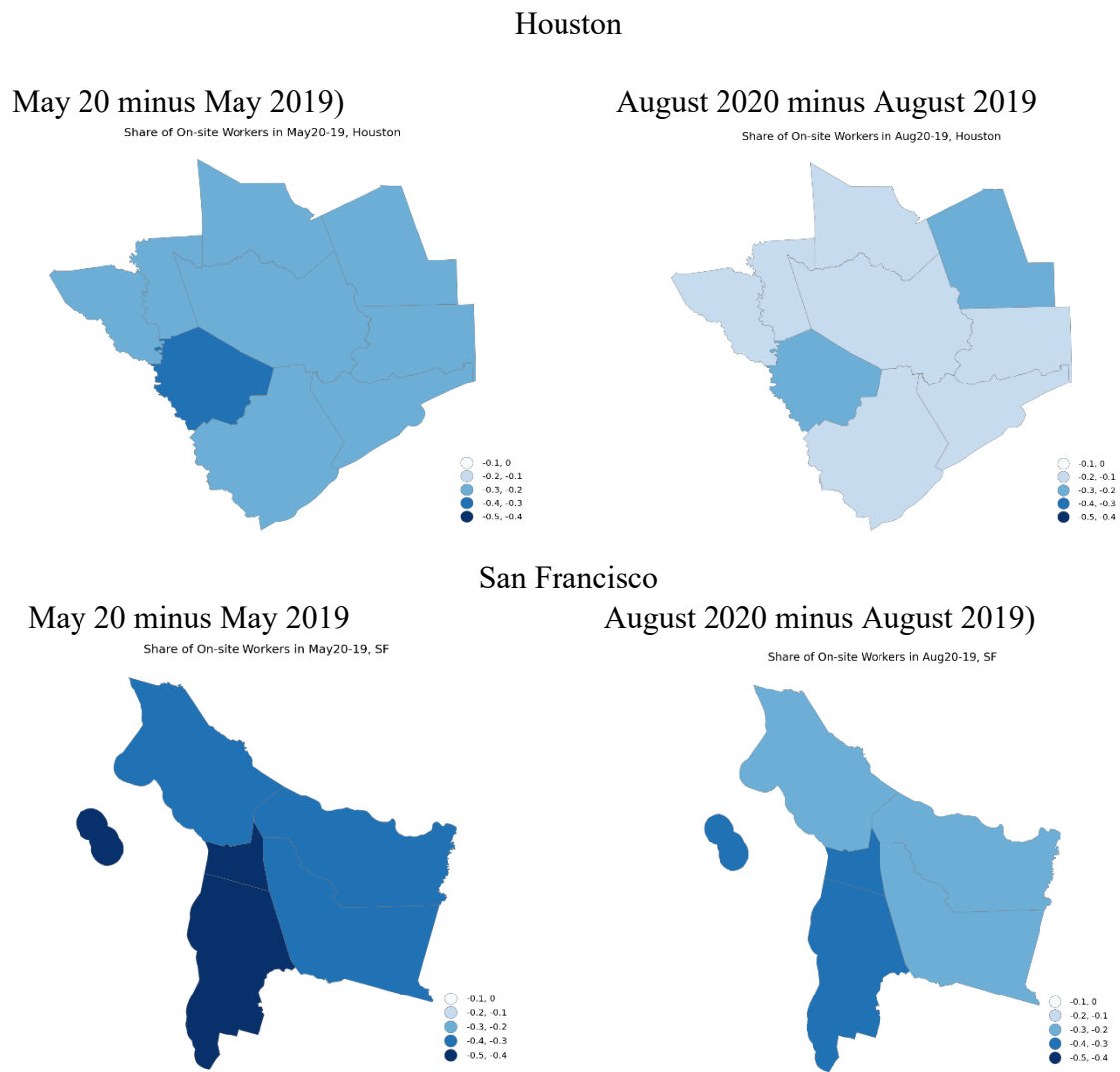
Figure 4: Difference in Share of Workers Persisting in Onsite Work from February, May 2020 minus May 2019 and August 2020 minus August 2019, Houston and San Francisco
