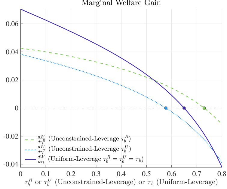
Figure 4: Uniform-Leverage-Regulation
