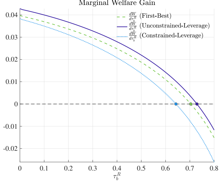
Figure 3: First-Best vs. Unconstrained-Leverage-Regulation vs. Constrained-Leverage-Regulation
