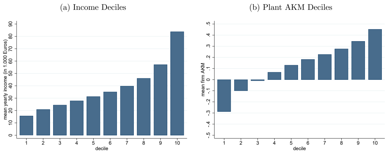
Figure A.3: Income and Plant AKM Distribution
