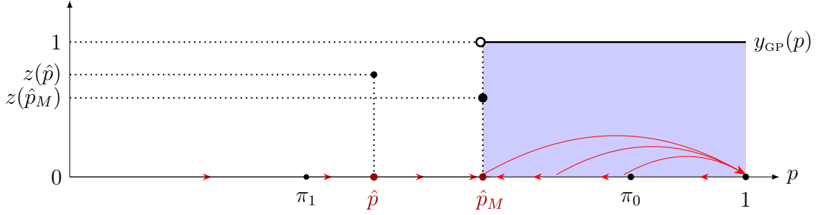
Figure 5: Enforcement Policy under MP: Case 3-b
