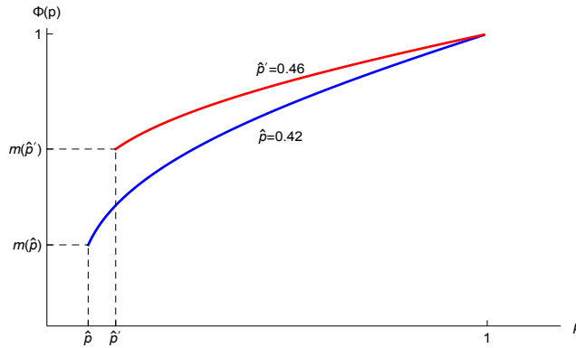
Figure 6: The invariant distribution of p under alternative cutoffs
