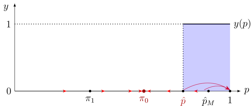
Figure 2: Low Crime Rates Case
