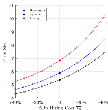
(b) Average Firm Size
