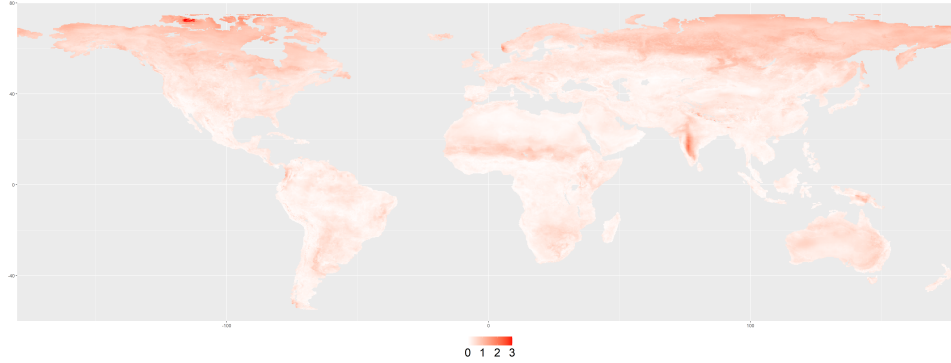
(c) RCP 6.0
