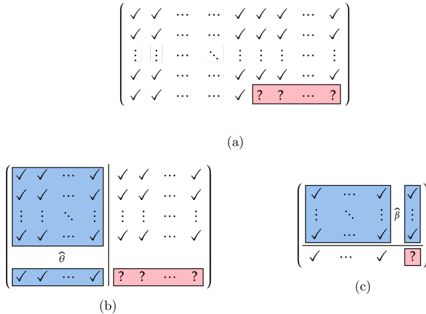
Figure 1: Problem statement and common estimators. Panel (a) illustrates the core challenge of imputing the counterfactual for the treated unit. Panels (b) and (c) respectively show the synthetic control and unconfoundedness approaches toward counterfactual estimation.
