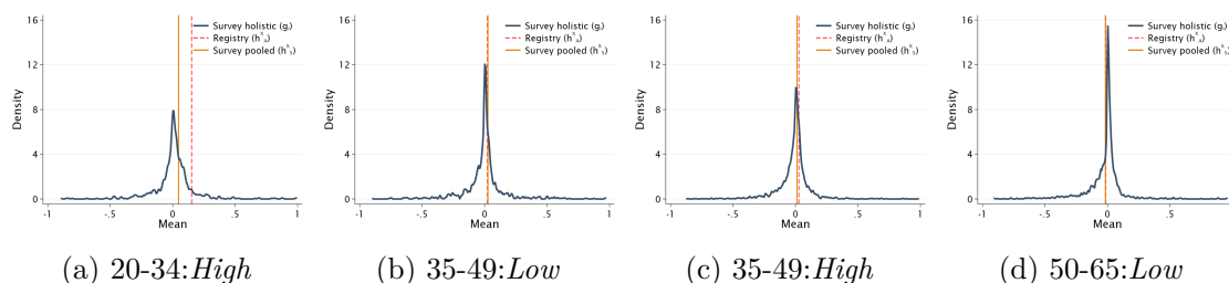
Figure E.1: Mean of h_S^X and h_A^X , and the distributions of individual means of g_i for four selected subgroups
