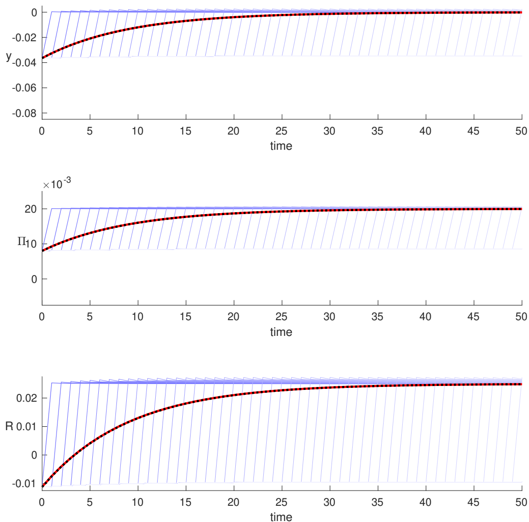
Figure 7: IRF and Contingencies - Outside the ZLB
