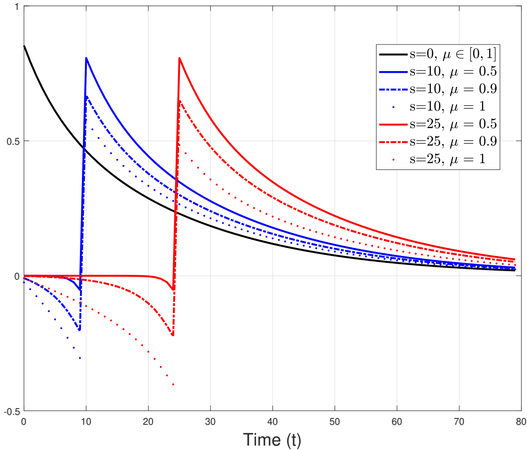
Figure 6: Asset Market Clearing Jacobian \left(\frac{dY_t^{\tau^{\max}-1}}{dY_s, t=0}\right) for Distinct \mu 's
