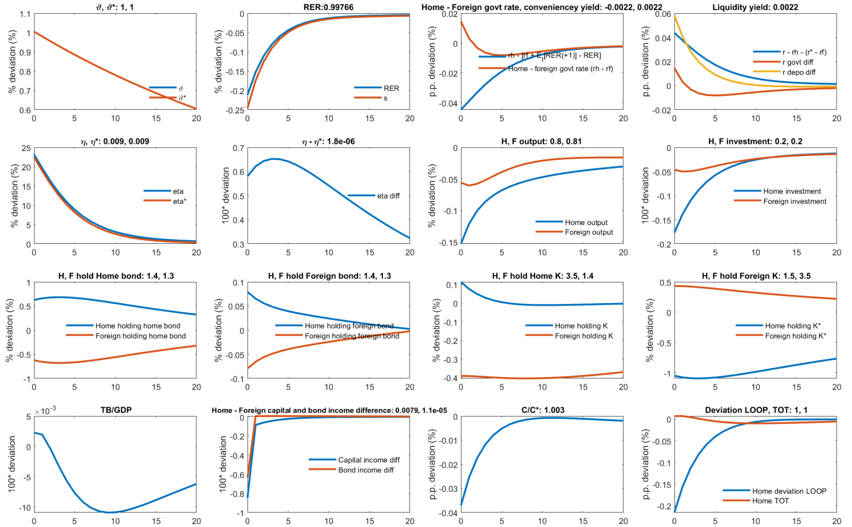
Figure 4: 1% global financial shock ( \vartheta, \vartheta^* ) with \kappa_{h1} = \kappa_{h1}^* = 0.025 < \kappa_{f1} = \kappa_{f1}^* = 0.32
