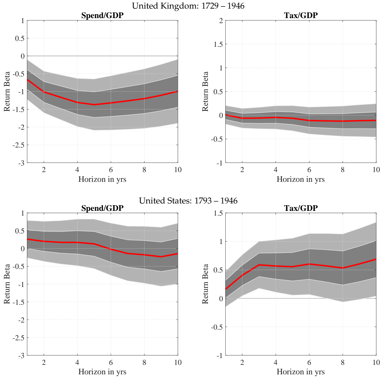
Figure A.3: Return Beta: Pre – 1946
