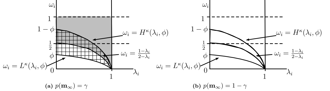
Figure 4: Fact-checking in mimicking equilibrium. Panel (a) shows behavior when receivers observe p(\mathbf{m}_\infty) = \gamma . Panel (b) shows behavior when receivers observe p(\mathbf{m}_\infty) = 1 - \gamma . In each panel: Only receivers whose priors lie in the hatched areas fact-check. Receivers whose priors lie in the gray areas would have chosen a_i = 1 in the base game.
