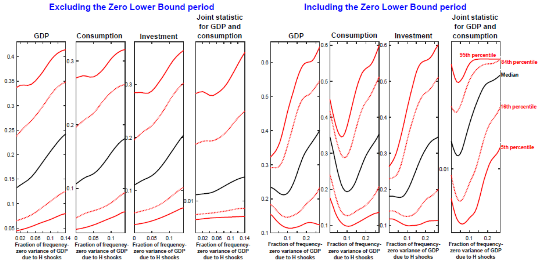
Figure 6 Median and selected percentiles of the Monte Carlo distribution of the Kolmogorov-Smirnov statistic
