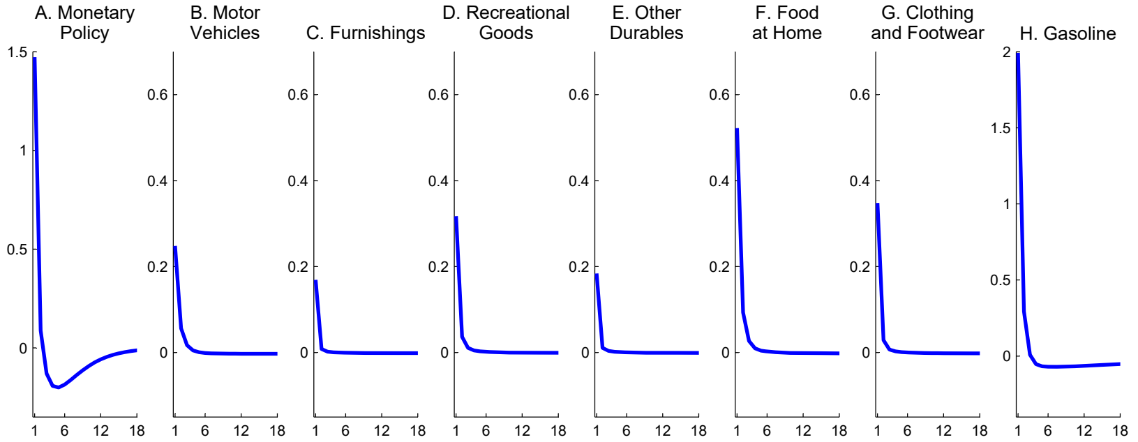
Figure 2: Inflation Responses
