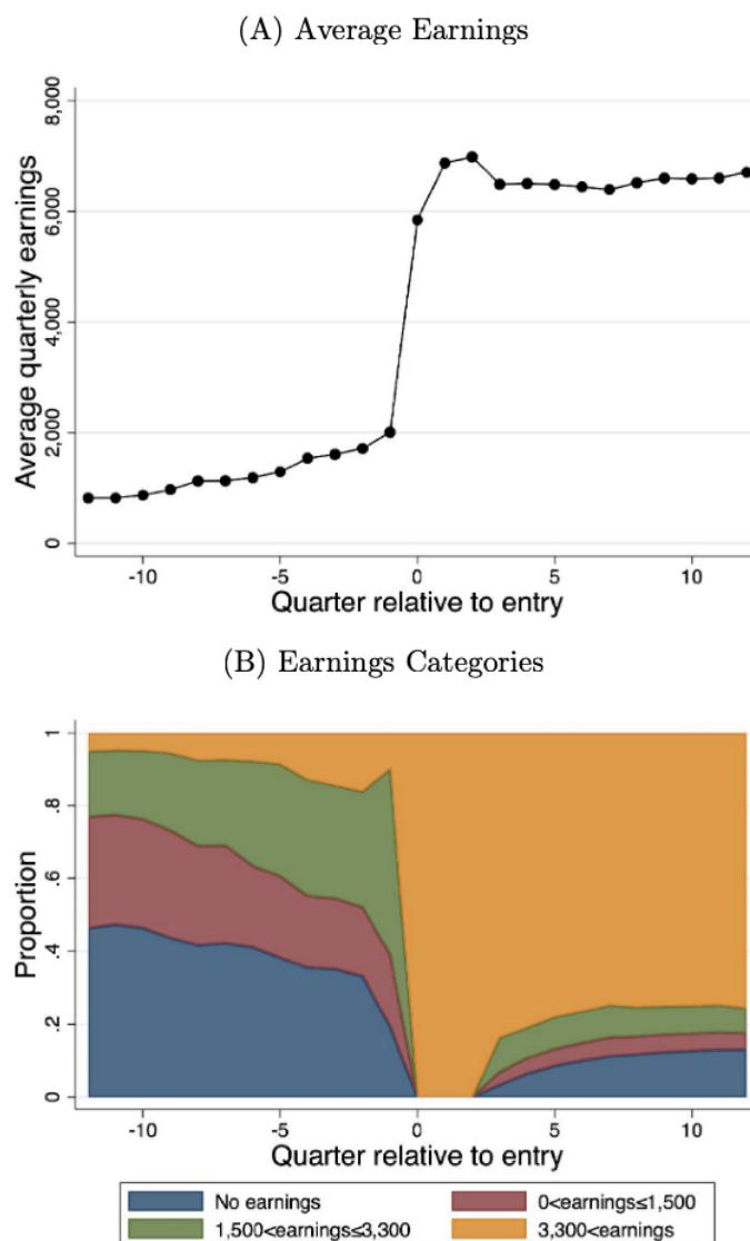
Figure A.1: Earnings Before and After Entry
