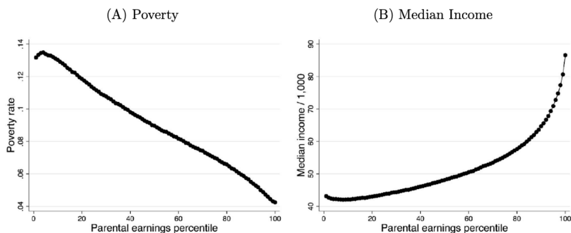
Figure B.4: Parental Earnings and Neighborhood Characteristics
