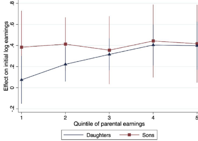
Figure 6: Heterogeneous Effects by Sex and Parental Earnings
