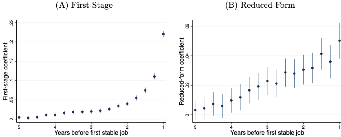
Figure 4: Hiring Rate in Earlier Years
