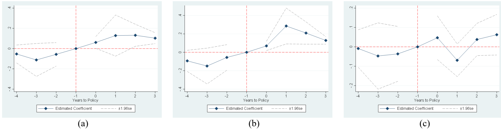
FIG. A.3. Tests of the parallel trend assumption in DID analysis. This figure shows the results from equation (16), which tests the validity of the parallel trend assumption in our DID specifications. The graphs plot the estimated \delta_\tau s along with the 95 percent confidence levels, which capture the savings rate impacts of the two-child policy in the \tau th year after the implement of the policy. \tau = -4, -3, -2, -1, 0, 1, 2, 3 is the distance between observation year and 2014 – the policy year. Year -1 is regarded as the base year, and the corresponding coefficient, \delta_{-1} , is set to 0. Panels (a)–(c) present the results for the whole matched sample, the female matched subsample, and the male matched subsample, respectively.
