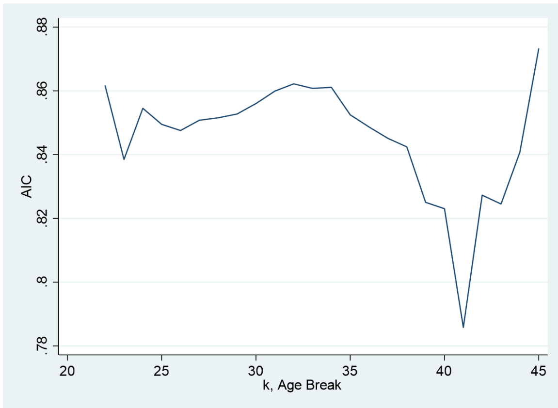
FIG. A.2.—The performance of the DID models about second-child fertility rate with different age breaks. This figure displays the performance of the DID models about second-child fertility rate, as discussed in Section V.A. Different age breaks (represented by symbol k in the equations) are used in the models, and the corresponding AICs are plotted.
