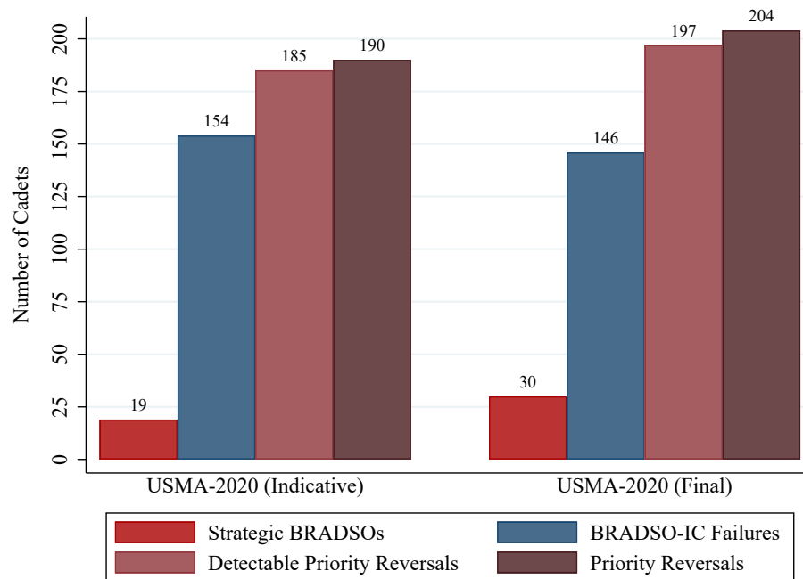
Figure 5: USMA-2020 Mechanism Performance under Truthful Strategies Simulated from Indicative and Final Preference Data from Class of 2021
