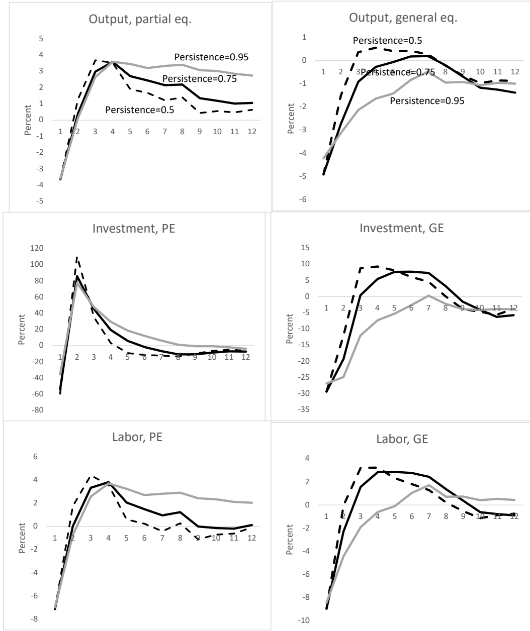
Figure A.1: IRFs in the RUBC model
