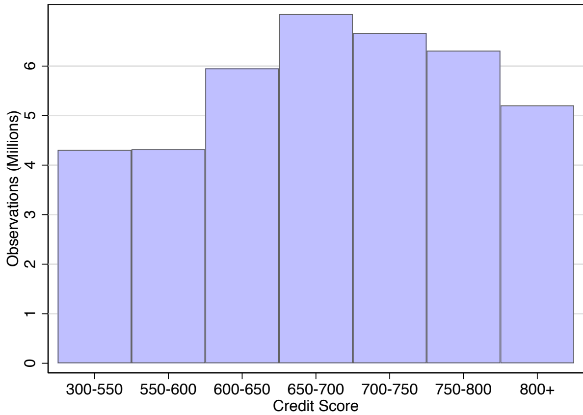
Figure A.4: Distribution of Credit Scores
