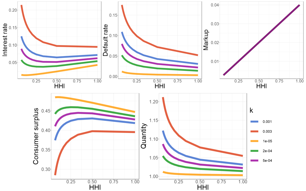
Figure 1: Model Simulations
