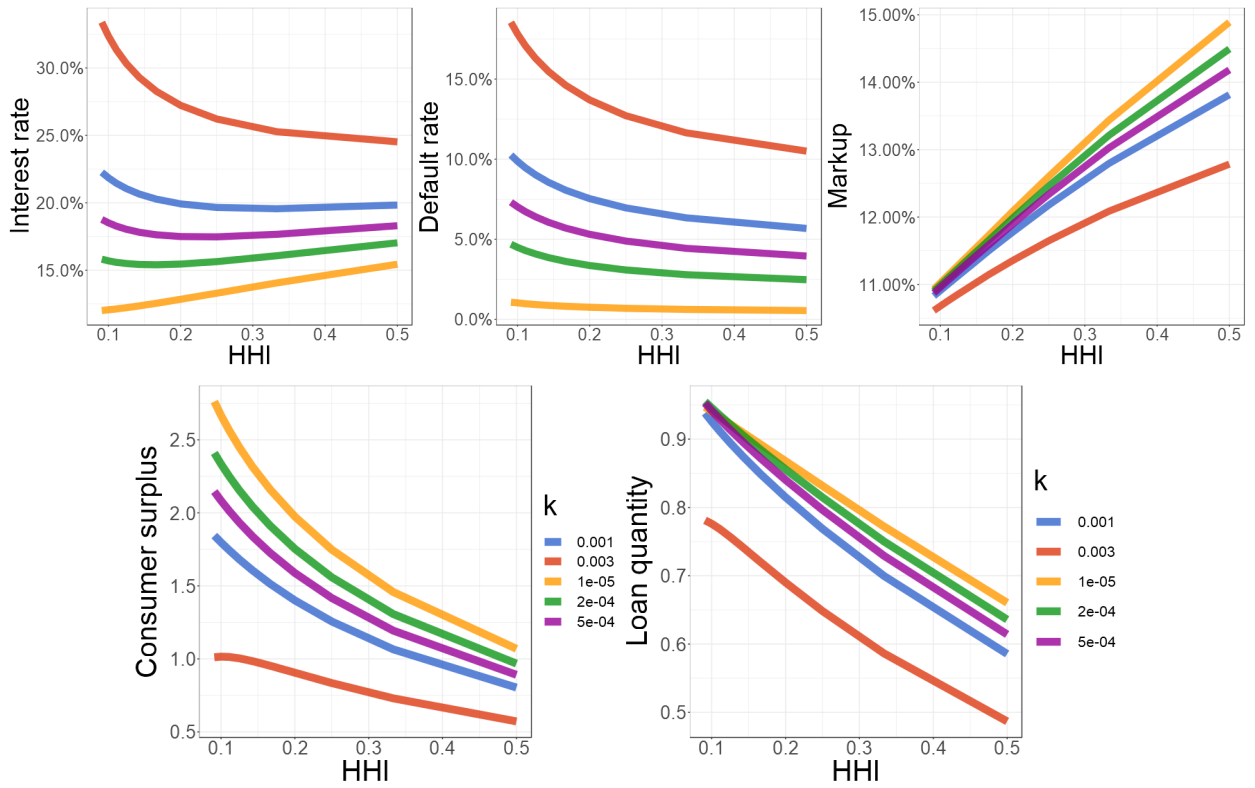
Figure A.1: Logit Model Simulations
