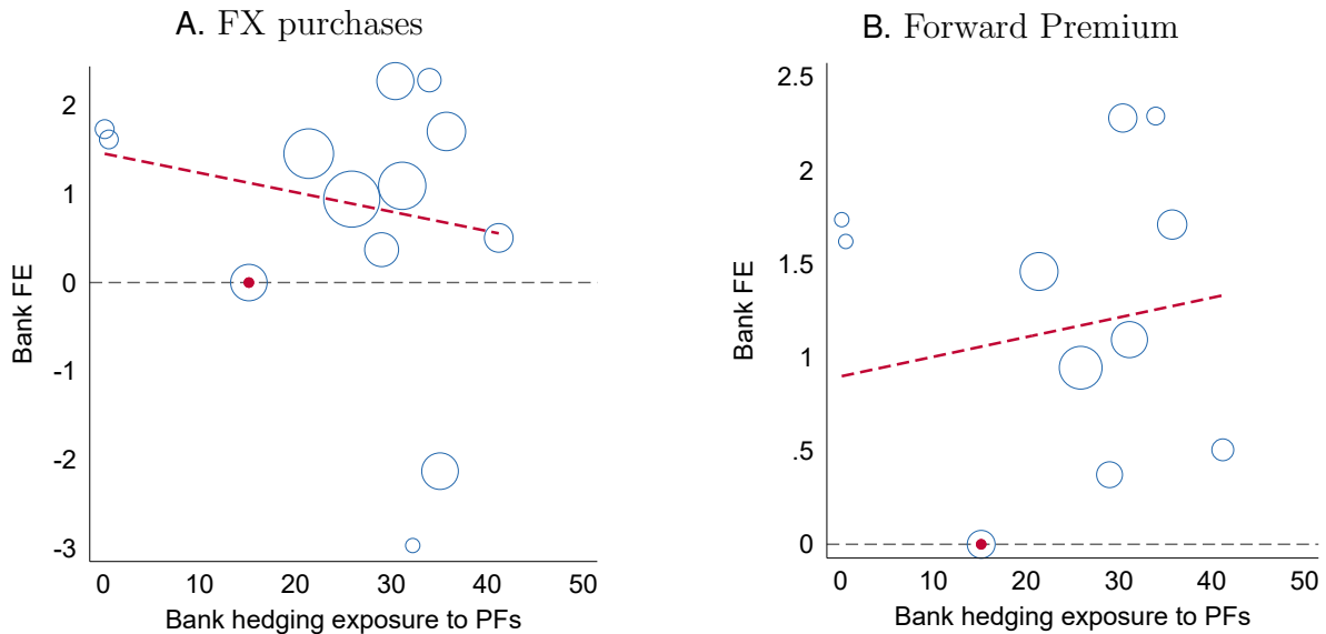
Figure A.7: Estimated supply shock in FX Premium and PFs in Banks' total FX purchases Note.— Vertical axis shows estimated bank fixed effects from equation (8), with dependent variable change in FX premium and the horizontal axis shows Pension Funds' share in each bank's total purchases of FX derivatives before the regulation change. Size of each circle represents share of bank in total purchases of FX derivatives from banks by firms. Red dashed line represents weighted linear fit.
