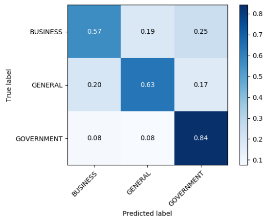
(b) Customers - Non-Binary
