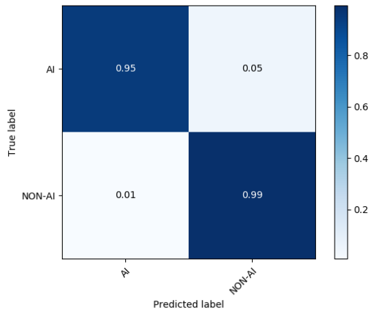
(c) Functions - Binary
