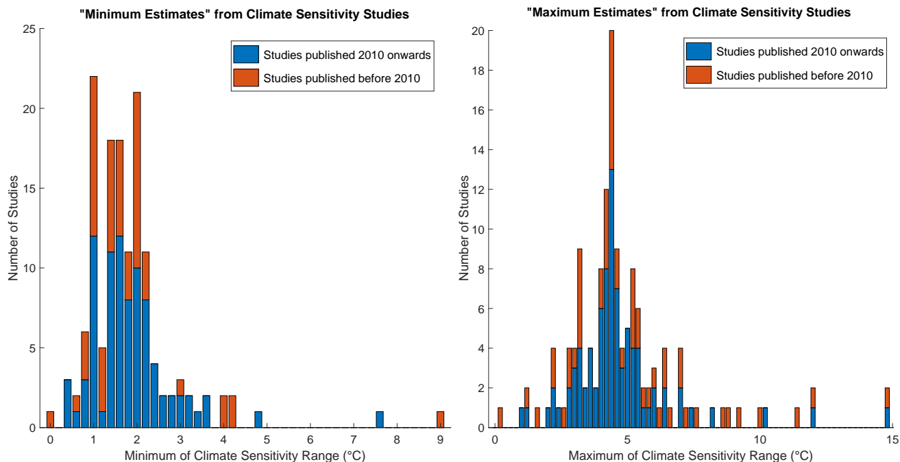
Figure 5: Histograms of Minimum and Maximum Estimates of Climate Sensitivity from from 143 studies, of which 54 were published prior to 2010 and 89 from 2010 onwards. The studies are from Knutti, Rugenstein and Hegerl (2017), supplemented by 9 additional studies published in 2017 and 2018, and listed in Footnote 11 on page 15..
