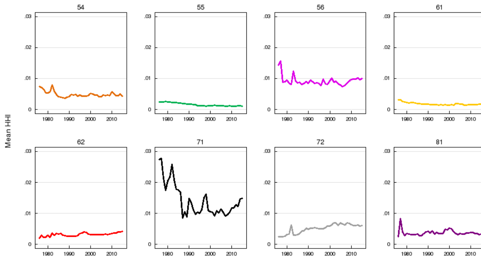
Figure B4: National Industrial Concentration Trends by Two-Digit NAICS Industry, Services, Excluding NAICS 51
