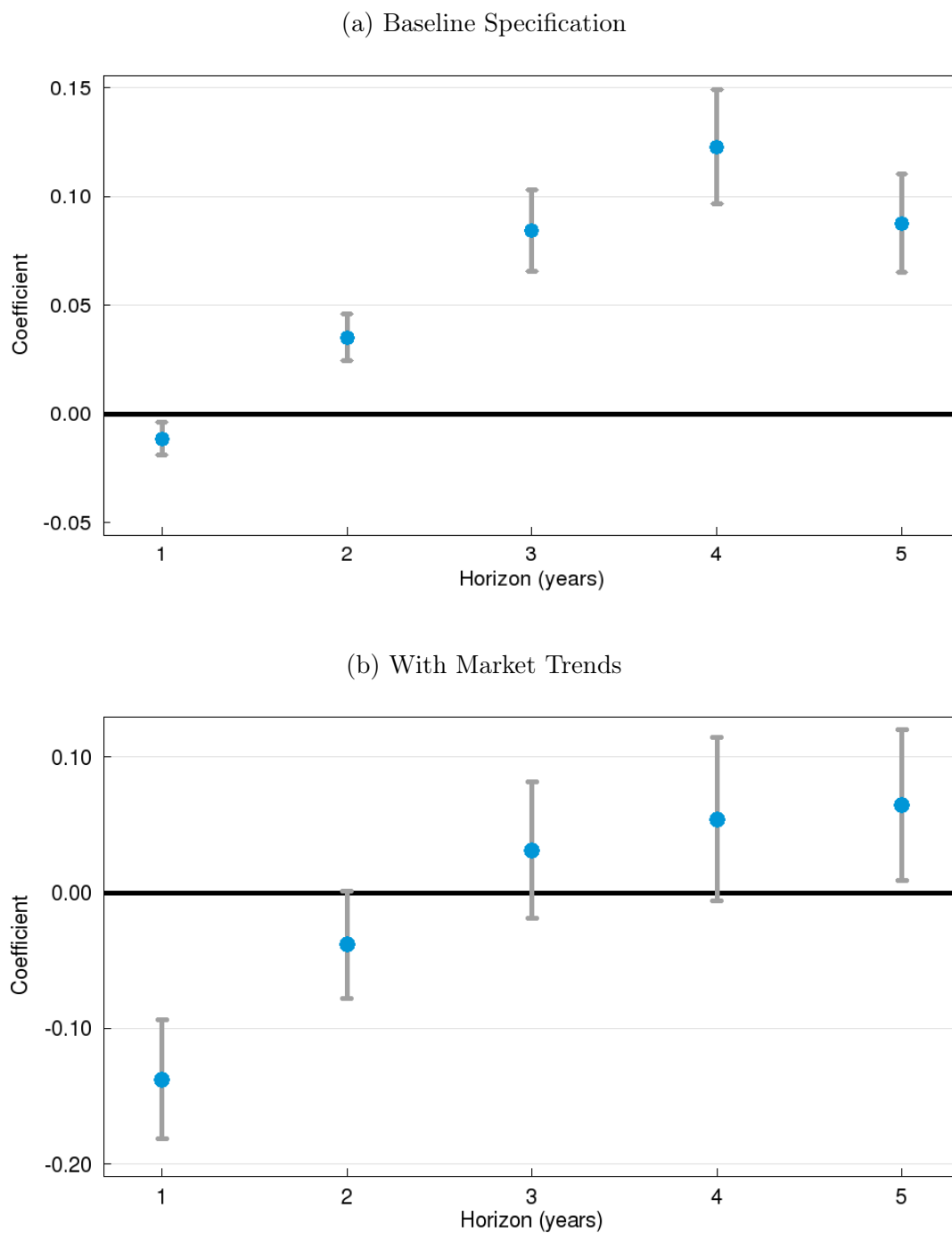
Figure 21: Effects of Industrial Concentration on Relative Earnings Mobility, by Length of Horizon
