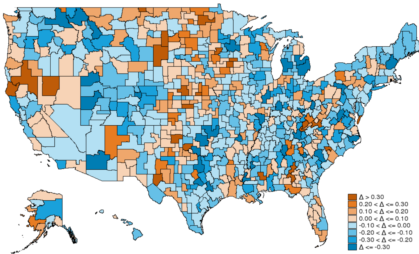
Figure 12: Changes in the Log of Average Concentration Across Industries within Commuting Zones, 1990–2005
