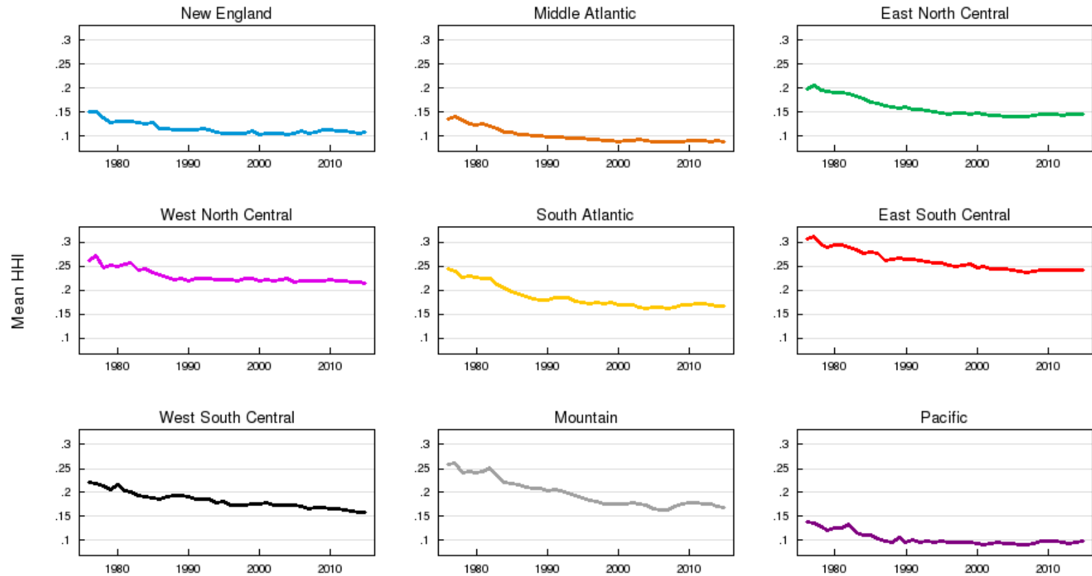
Figure B14: Local Industrial Concentration Trends by Census Division
