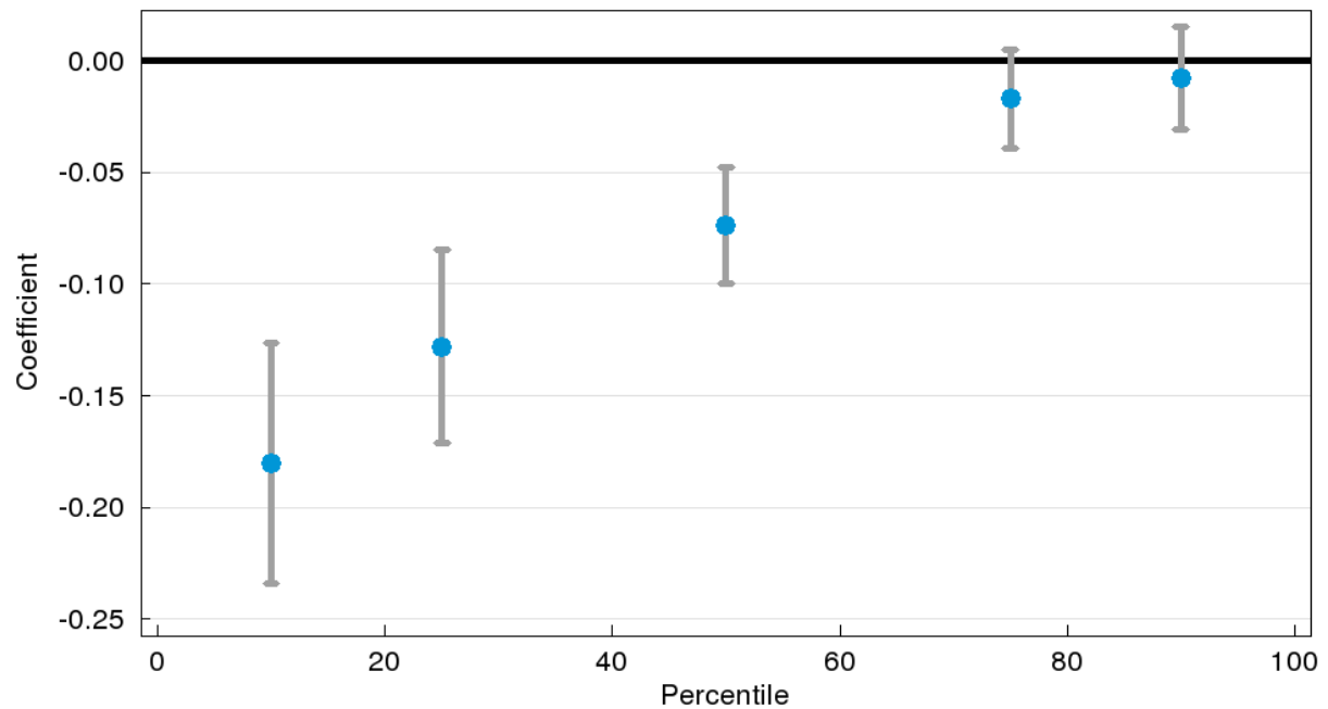
Figure 16: Effects of Industrial Concentration on Key Percentiles of the Earnings Distribution
