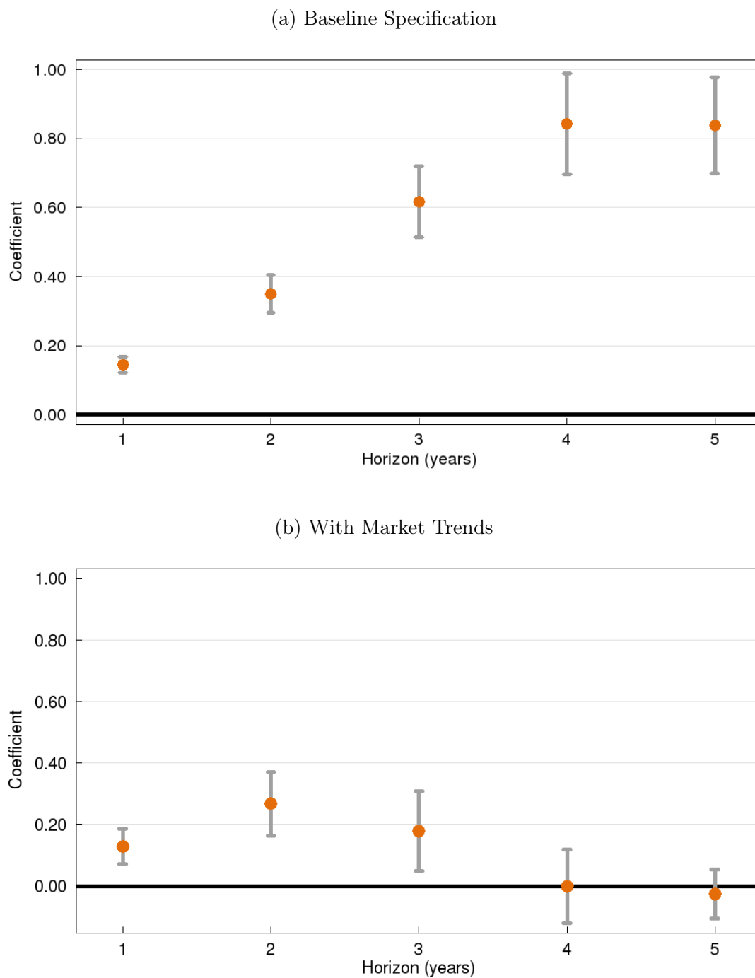
Figure 22: Effects of Industrial Concentration on Absolute Earnings Mobility, by Length of Horizon
