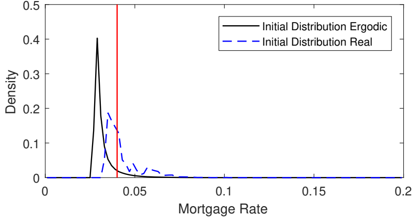
Figure 11: Distribution of m^* in Ergodic and Actual Simulation
