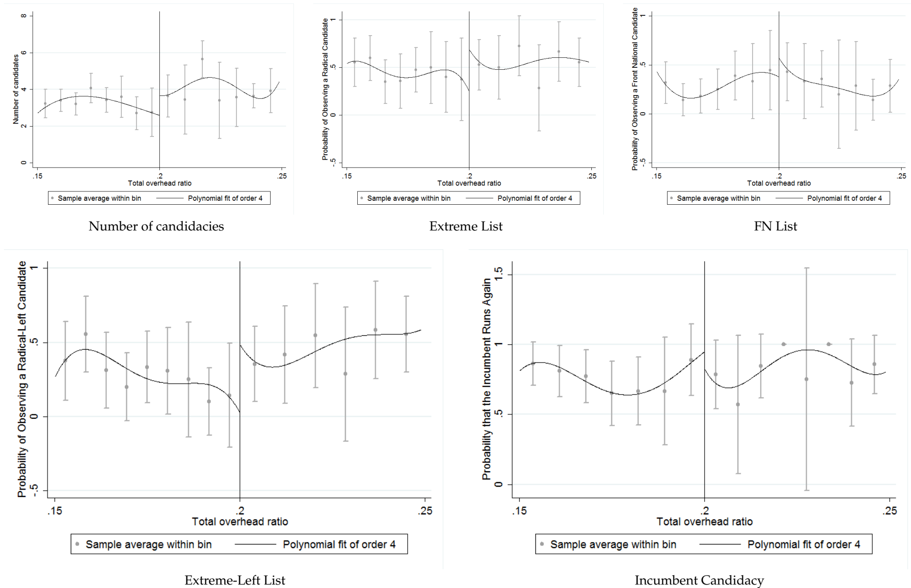
Figure 6: Regression Discontinuity Design: 20% threshold of the overhead ratio (Orange to Red)
