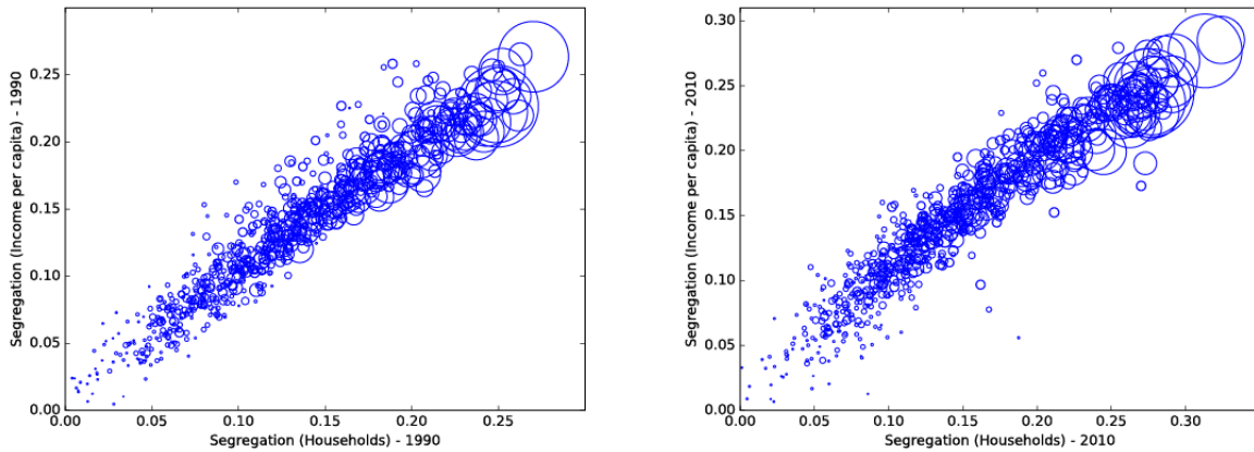
Figure A.1: Correlation between Segr_{CZ} computed using the approximated distribution of household income (horizontal axis) and the actual distribution of average personal income across CTs (vertical axis) in 1990 (left panel) and 2010 (right panel).
