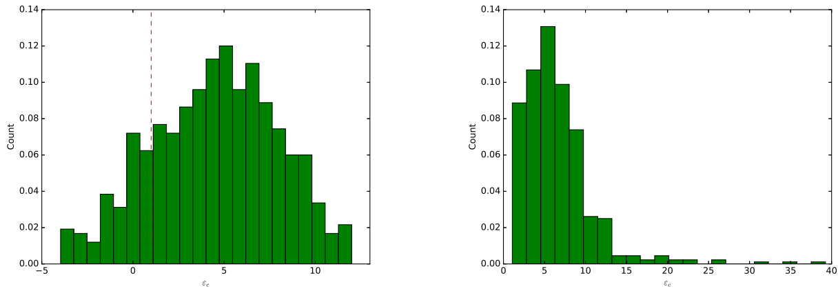
Figure D.1: The two histograms show the distribution of \epsilon_c estimated through a 2SLS procedure that uses a model-generated instrument. The left histogram reports the entire distribution after dropping the top and bottom 5% of the values. The right panel reports the distribution for \epsilon_c > 1 only.
