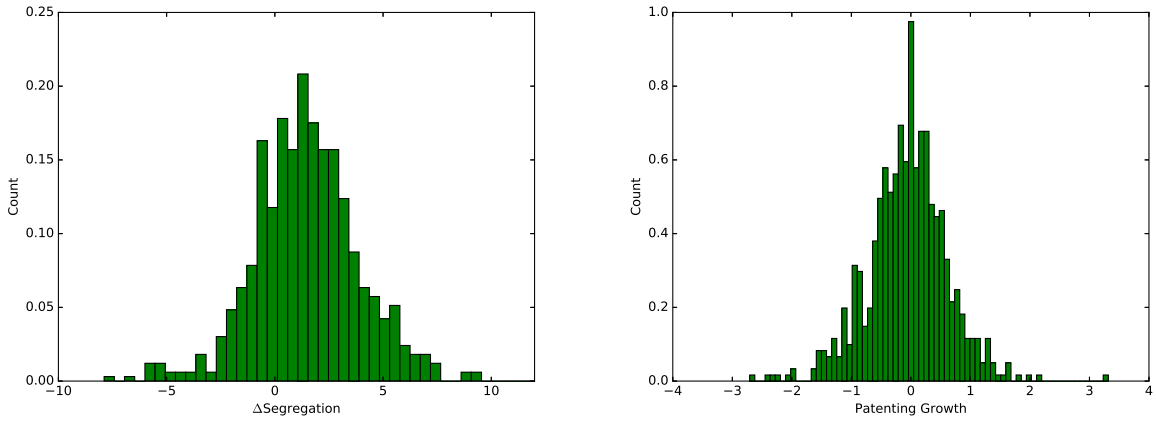
Figure B.1: Distribution of changes in measured segregation and patenting growth in the cross section of U.S. CZs, 1990-2010.
