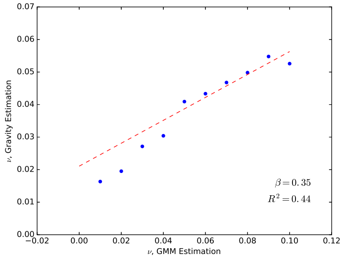
Figure B.5: The bin scatter plot compares the value of \nu_c estimated using (4.16) with the value of \nu_c that minimizes the difference between the share of people in city c commuting for less than 60 minutes and the model generated counterpart.
