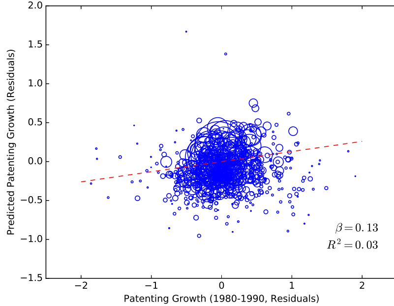
Figure B.2: Scatter plot of predicted patenting growth (instrument) and pre-trend in patenting (1980-1990). The scatter plot is weighted by total households in 1990.
