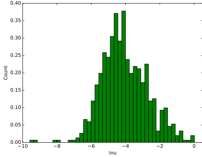
Figure B.4: Distribution of estimated values of \nu_c in U.S. commuting zones
