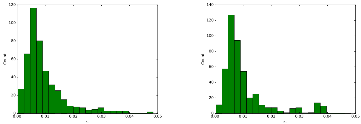
Figure D.2: The two histograms report the distribution of \kappa_c for those commuting zones with \epsilon_c > 1 . The left and right histograms show the unweighted and weighted distribution of this variable, respectively.
