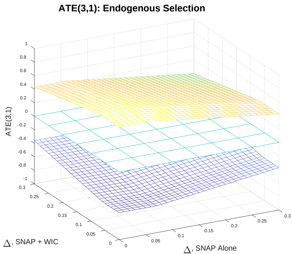
Figure 1. Bounds on ATE_{31} under Endogenous Selection
