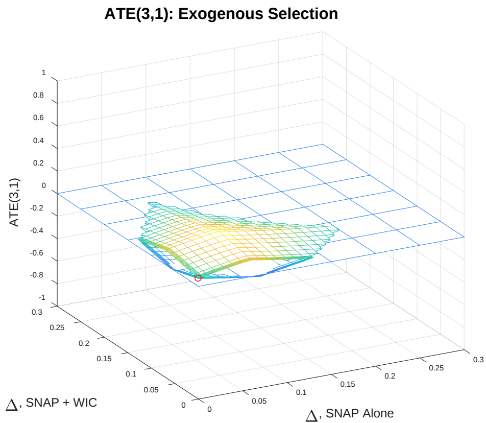
Figure 2. Bounds on ATE_{31} under Exogenous Selection
