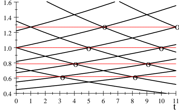
Figure 4: The circles in the figure are pairs (\pi_k, t) which belong to the same wave r and two consecutives periods n and n' = n + 1 .
