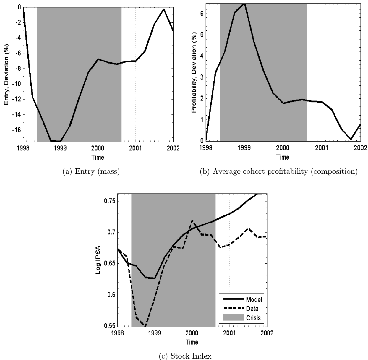
Figure 2: Model Performance
