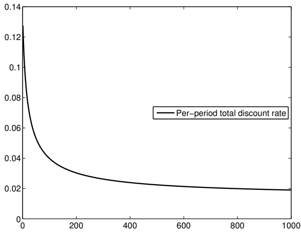
(c) Hyperbolic-Exponential
