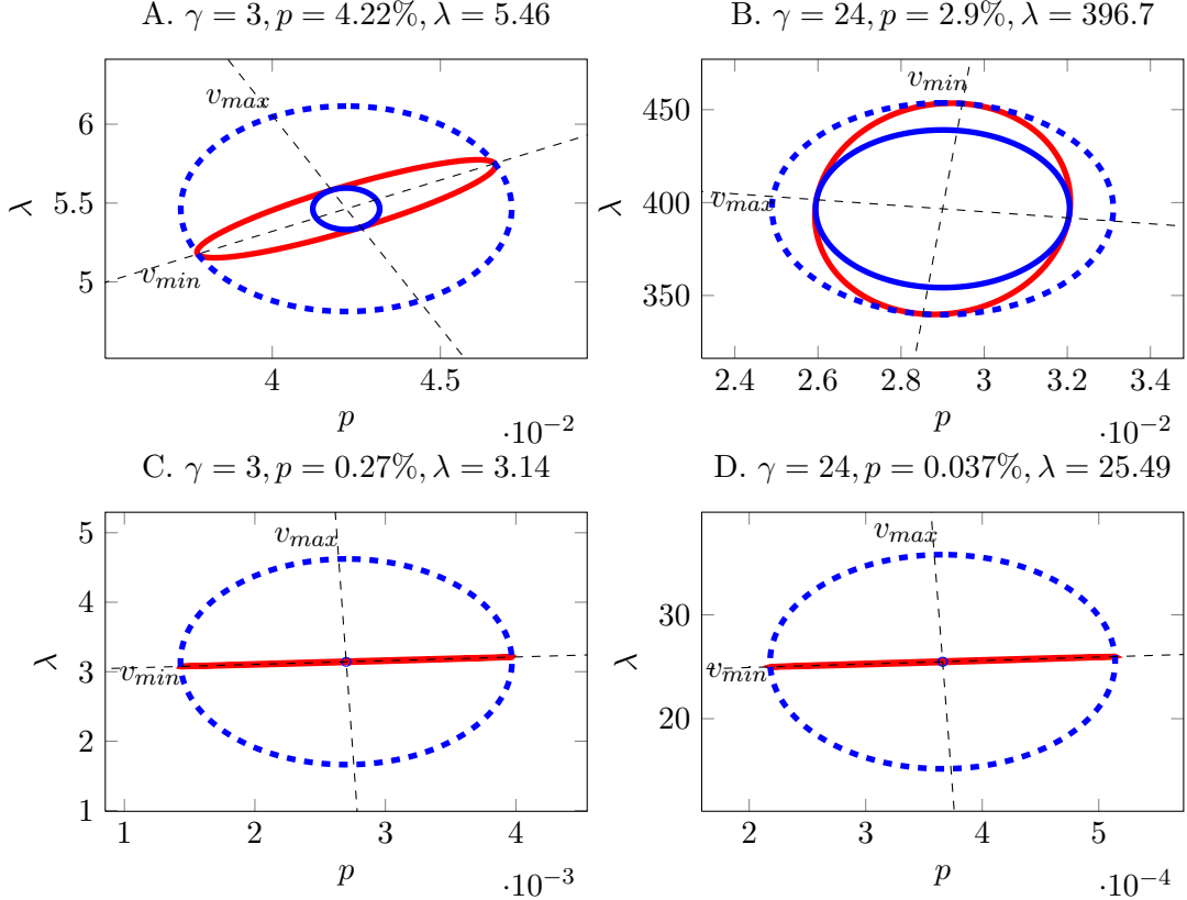
Figure 4: The 95% confidence regions for the asymptotic distributions of the MLEs for four “acceptable calibrations.” In Panels A through D, the asymptotic information ratios are \rho_a(\mu, \sigma^2) = 24.47, 1.81, 3.7 \times 10^4, \text{ and } 2.9 \times 10^4 .
