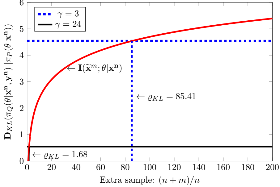
Figure 9: Computing the finite sample information ratio. The two horizontal lines represent the relative entropy between the constrained and unconstrained posterior on \theta for \gamma = 3 and 24. Their intersections with the conditional mutual information \mathbf{I}(\tilde{\mathbf{x}}^m; \theta | \mathbf{x}^n) mark the value of the finite sample information ratio \varrho_{KL} .
