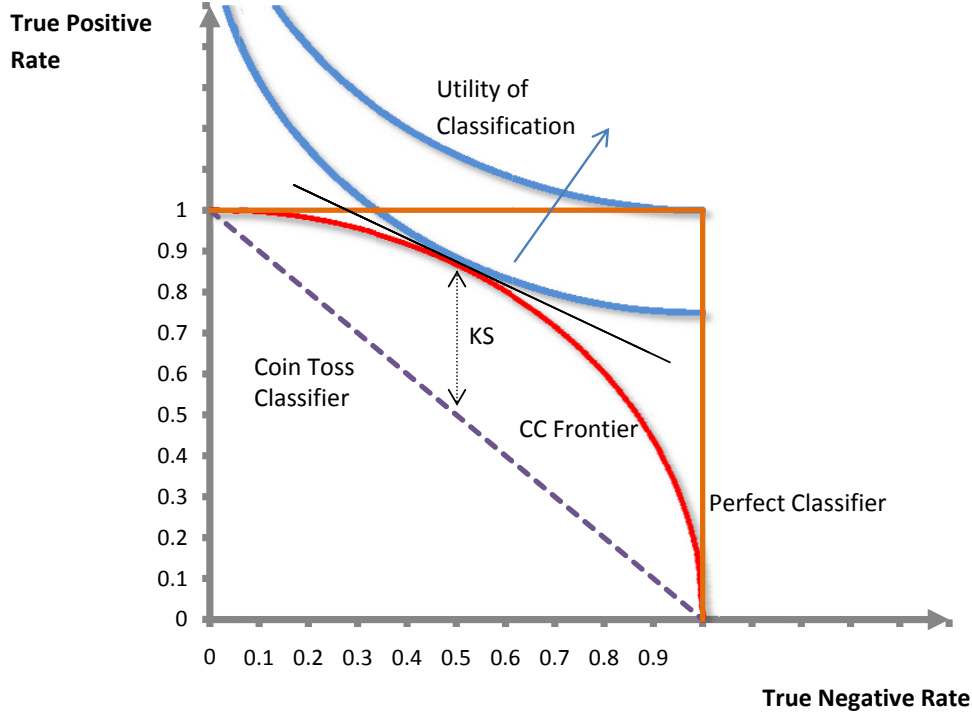
Figure 1: The Correct Classification Frontier
