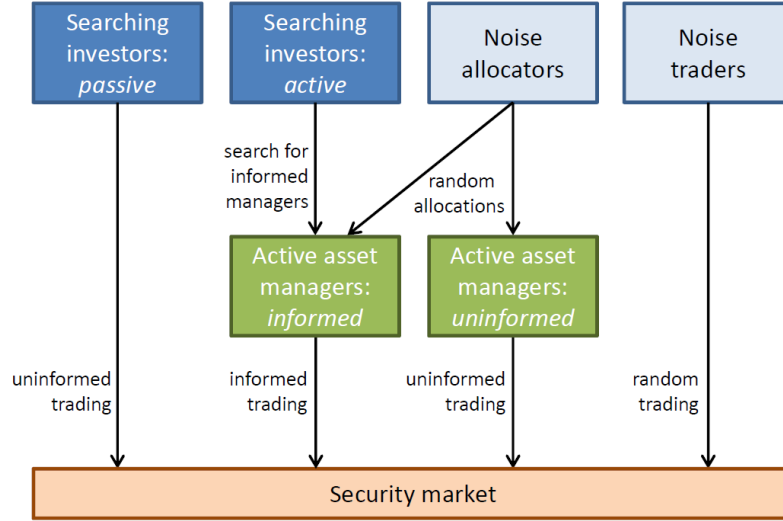
Figure 1: Model Overview.
