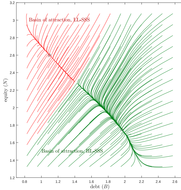
Figure 7: Convergence paths.
